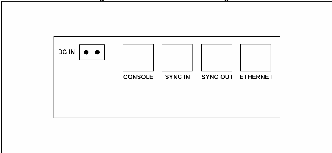
Figure 5. SEM2411X Rear Panel
