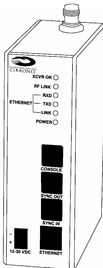
Figure 3. SEM2411D Front Panel Diagram
