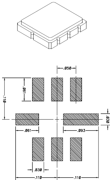
PCB Foot Print Dimensions in Nominal Inches
