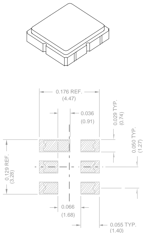
PCB Footprint
