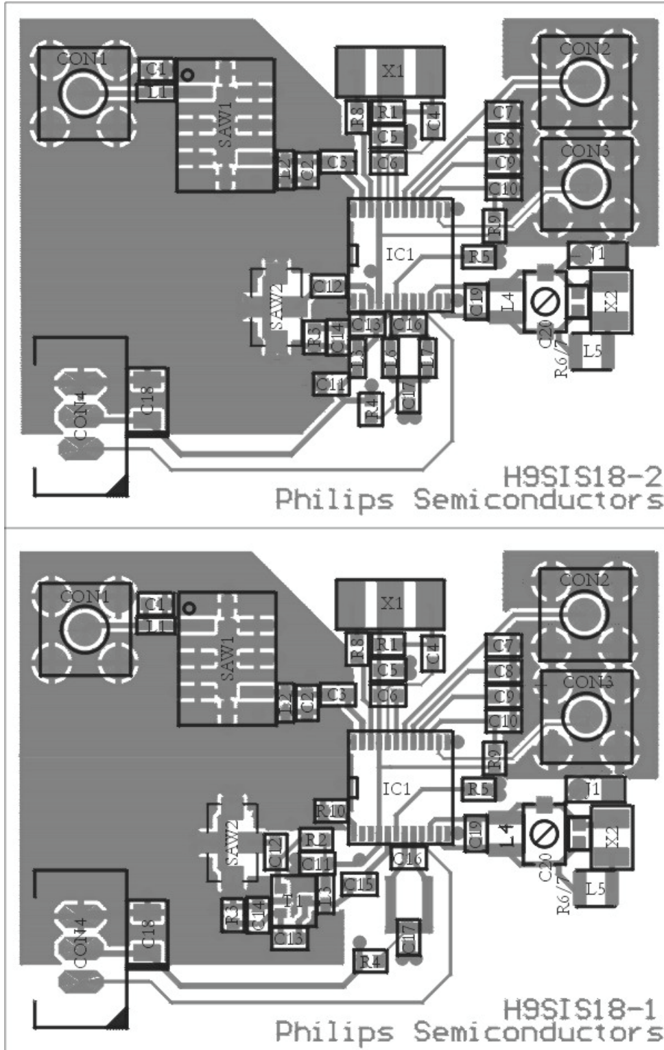
Figure 6: H9SIS18-1/2 layout and component placement, top side
