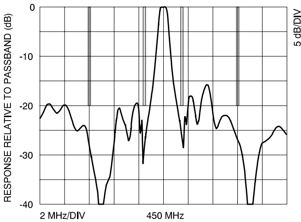
Figure 10: Typical SAW CR Response (continued)
