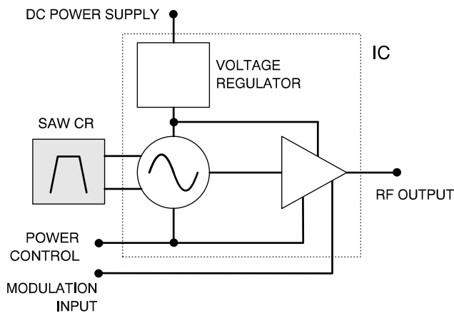
Figure 19: The Microtransmitter
