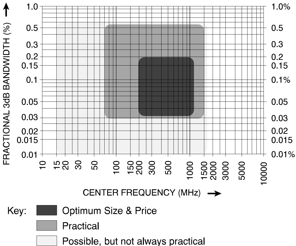
Figure No. 4: Frequency and Bandwidth Capabilities
